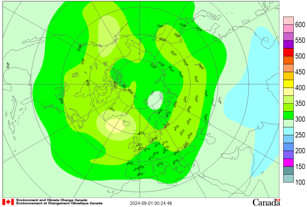
Mean total ozone (DU), 2024/08/01-2024/08/31
