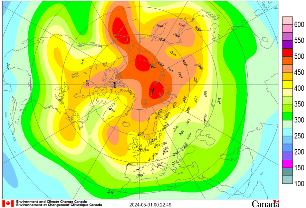
Mean total ozone (DU), 2024/04/01-2024/04/30
