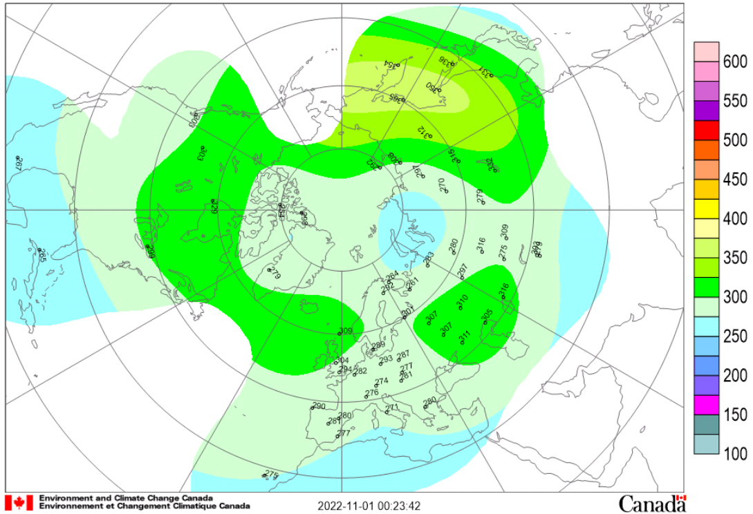
Mean total ozone (DU), 2022/10/01-2022/10/31
