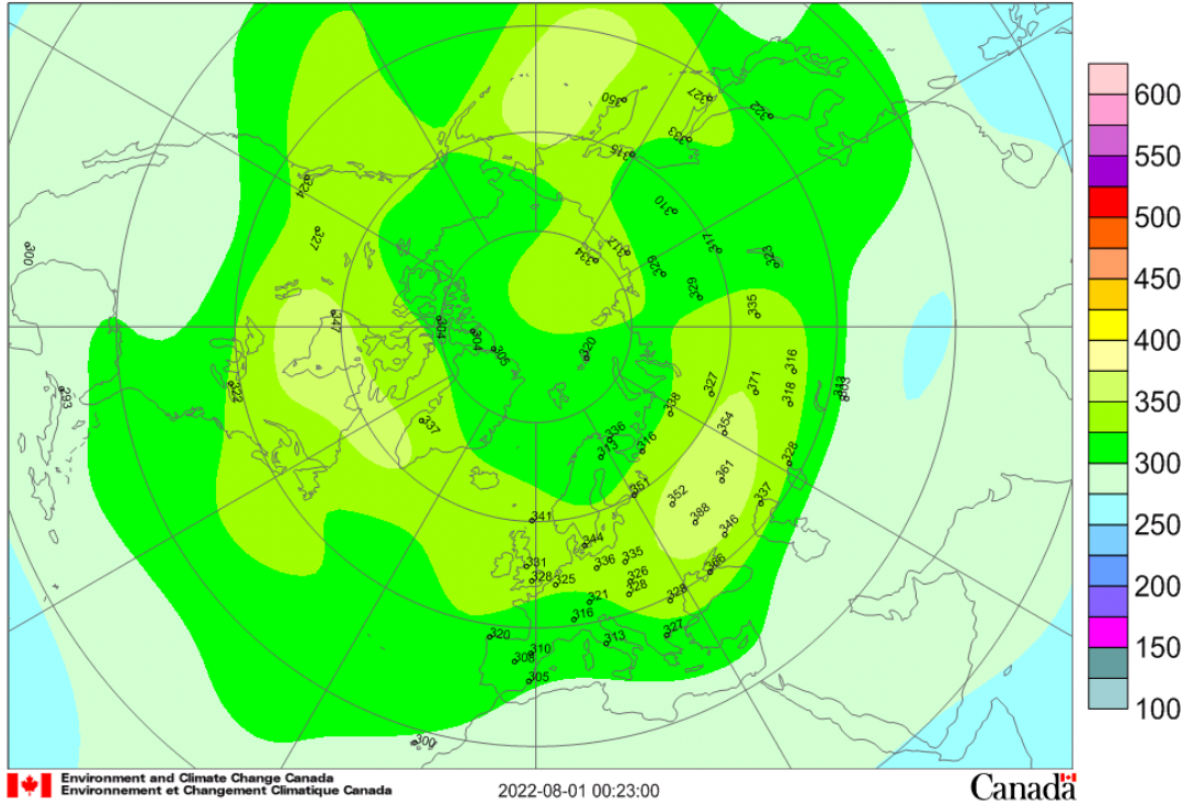
Mean total ozone (DU), 2022/07/01-2022/07/31
