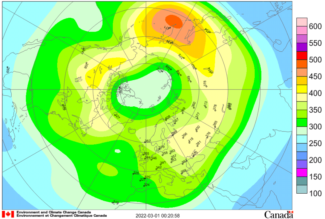
Mean total ozone (DU), 2022/02/01-2022/02/28
