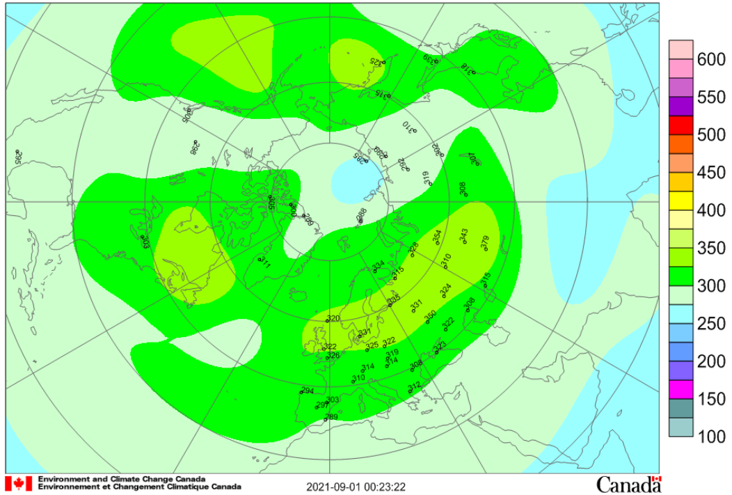
Mean total ozone (DU), 2021/08/01-2021/08/31
