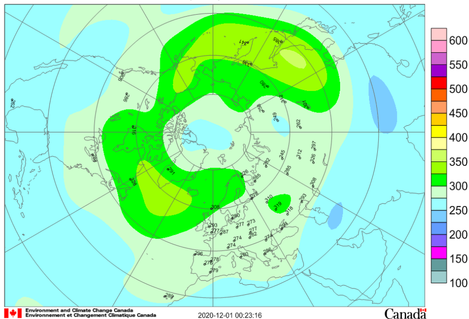
Mean total ozone (DU), 2020/11/01-2020/11/30
