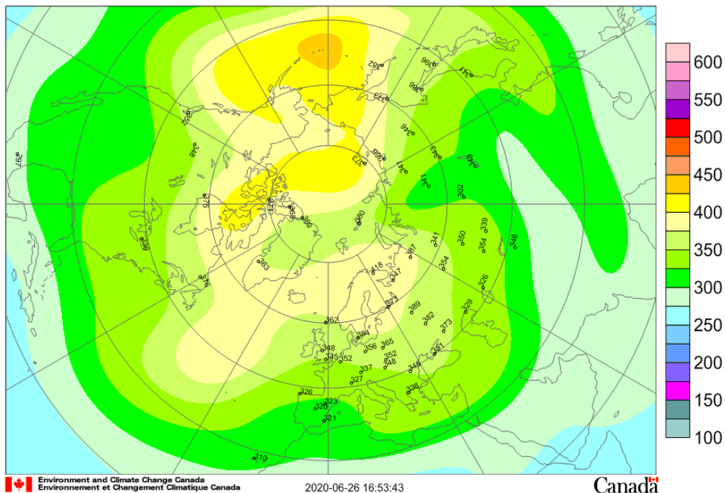
Mean total ozone (DU), 2020/05/01-2020/05/31
