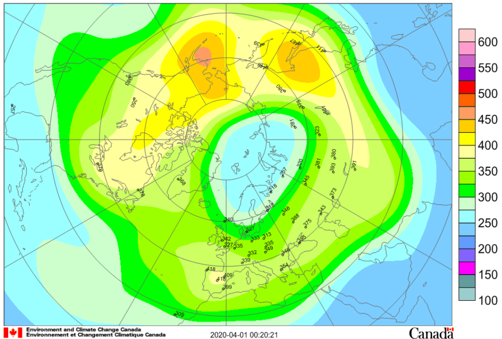
Mean total ozone (DU), 2020/01/01-2020/01/31
