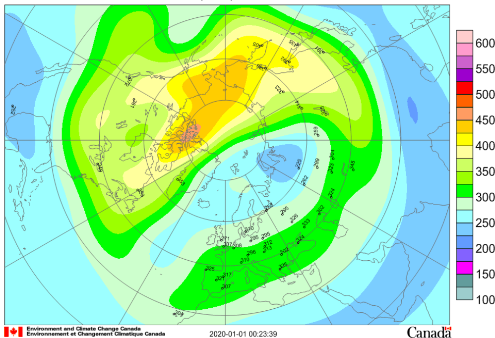
Mean total ozone (DU), 2019/12/01-2019/12/31
