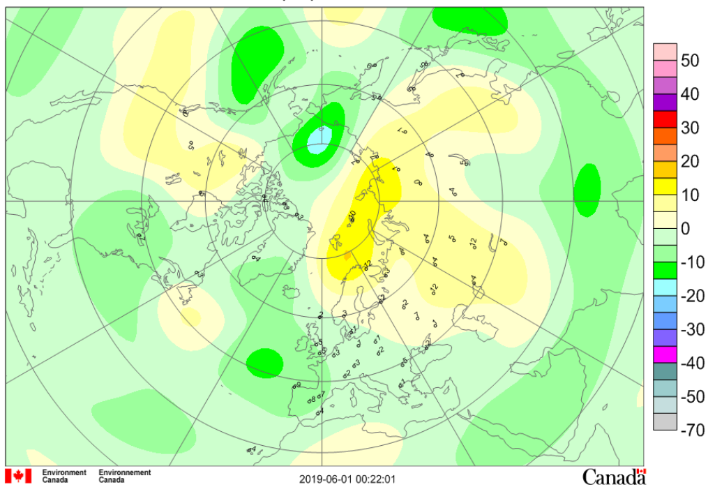
Mean deviation (%), 2019/05/01-2019/05/31
