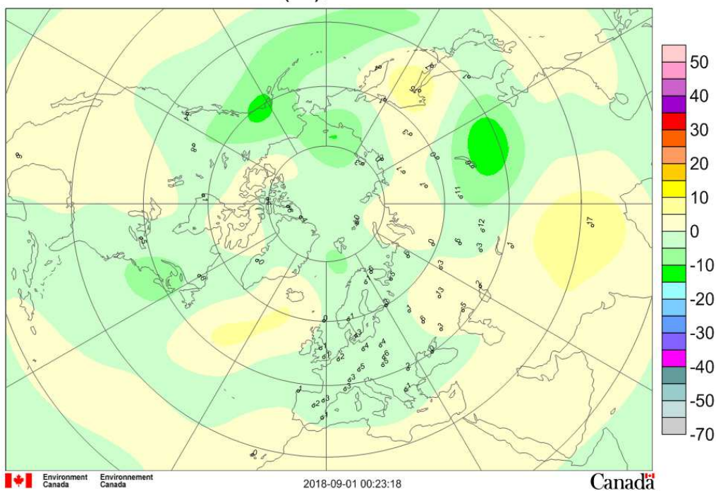
Mean deviation (%), 2018/08/01-2018/08/31
