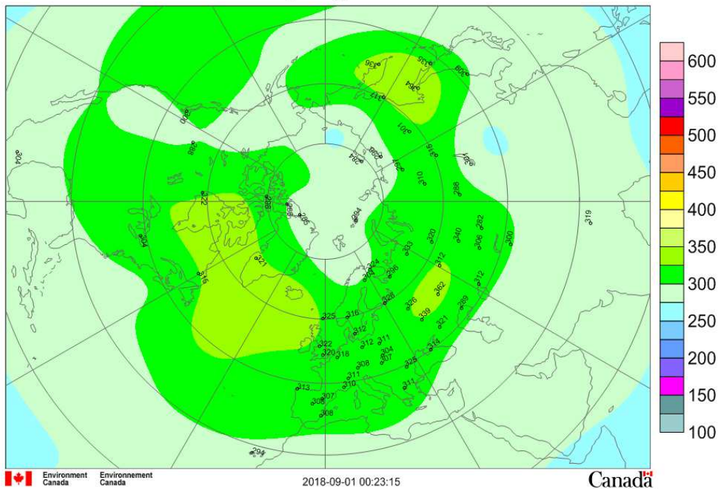
Mean total ozone (DU), 2018/08/01-2018/08/31
