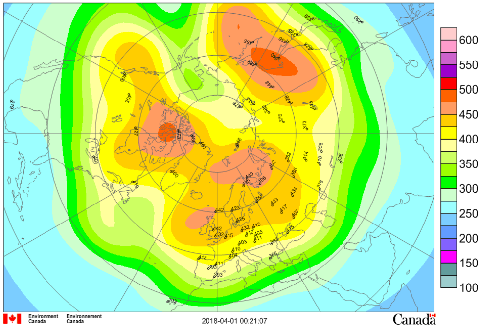
Mean total ozone (DU), 2018/03/01-2018/03/31
