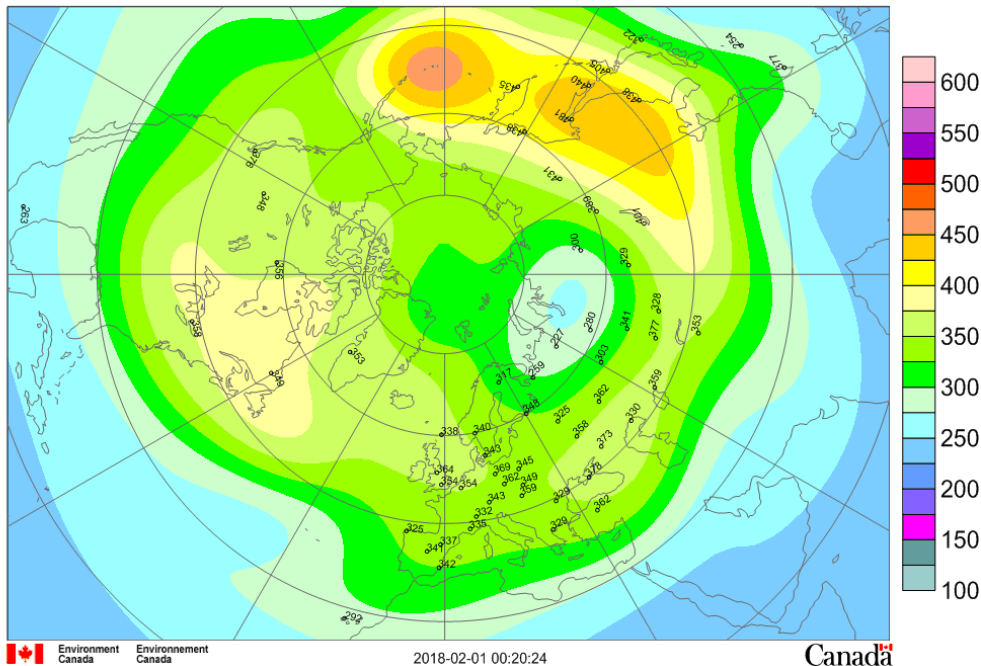
Mean total ozone (DU), 2018/01/01-2018/01/31
