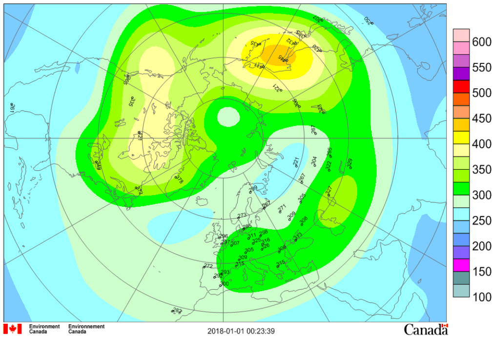
Mean total ozone (DU), 2017/12/01-2017/12/31
