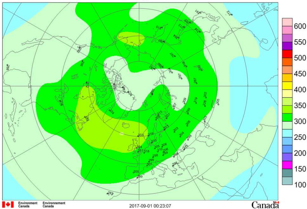
Mean total ozone (DU), 2017/08/01-2017/08/31
