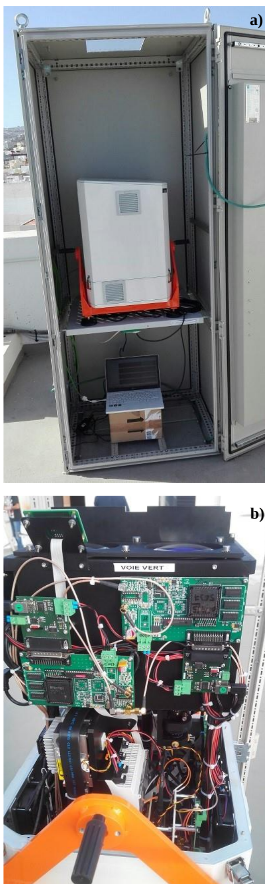
Figure 9.3 The new Cimel CE376 lidar: a) in the thermostated enclosure on the Santa Cruz Observatory instrument terrace and b) different details of the instrument.
