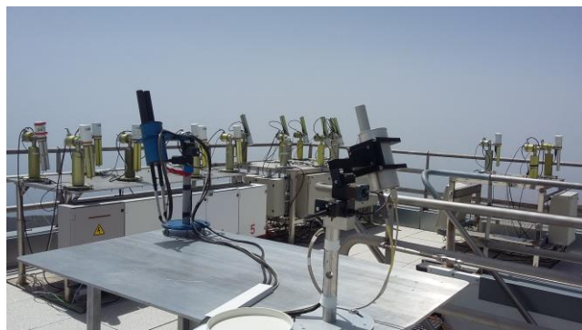
Figure 21.7. The original Pandora (in the foreground), the new Pandora-2S and several Cimel photometers (background).
