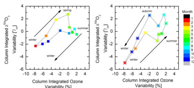
Figure 7.5. Intra-annual variability of the \{\delta^{50a}\text{O}_3, {}^{48}\text{O}_3\} and \{\delta^{50s}\text{O}_3, {}^{48}\text{O}_3\} pairs as observed by the IARC FTIR. Reprinted from Sanromá et al. (2016).
