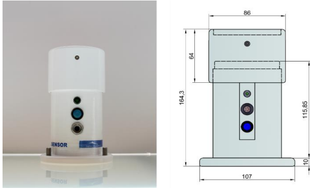
Figure 22.5. ZEN-R41 scheme and dimensions.
