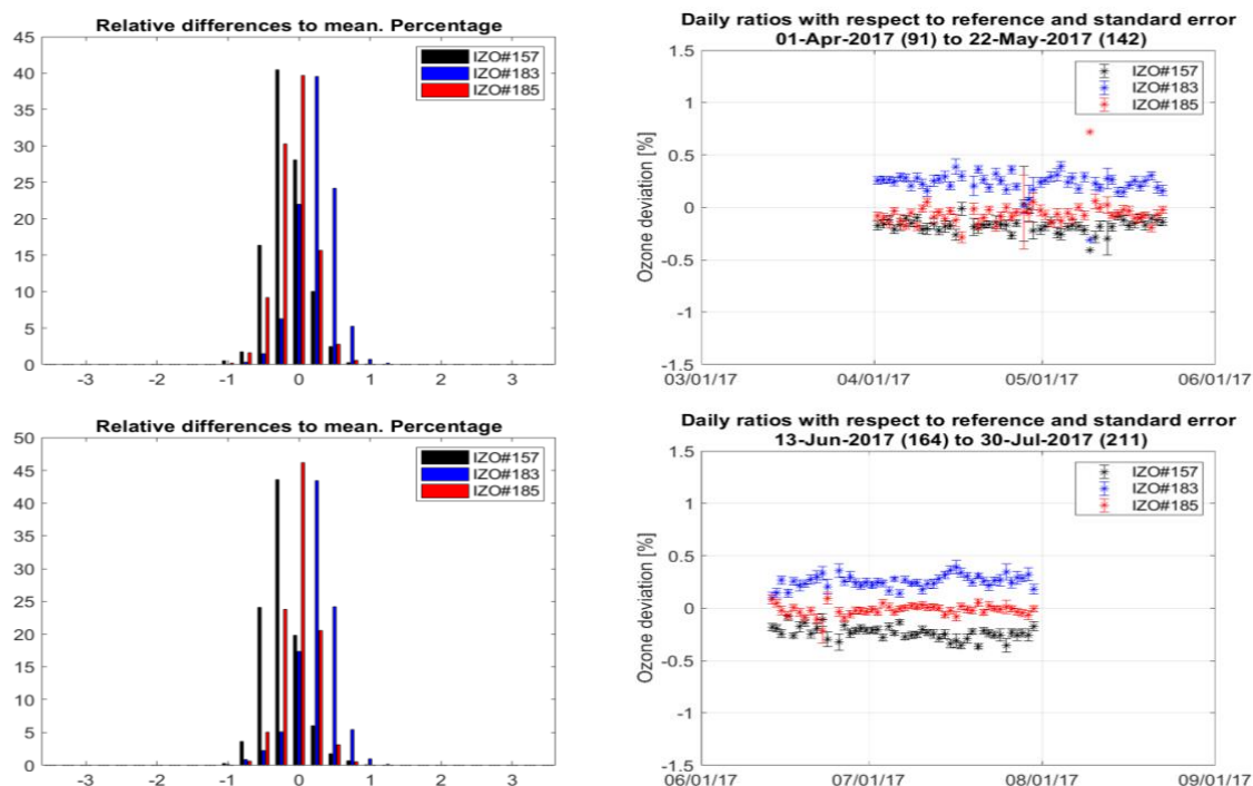
Figure 12. Deviations of near-simultaneous ozone measurements of RBCC-E standard Brewer (serial no. #157, #183 and #185) to the triad mean (left) and temporal evolution of daily mean deviation of near-simultaneous ozone measurements with the error bars representing the standard error (right). Data before (top) and after (bottom) the El Arenosillo 2017 intercomparison are presented.
