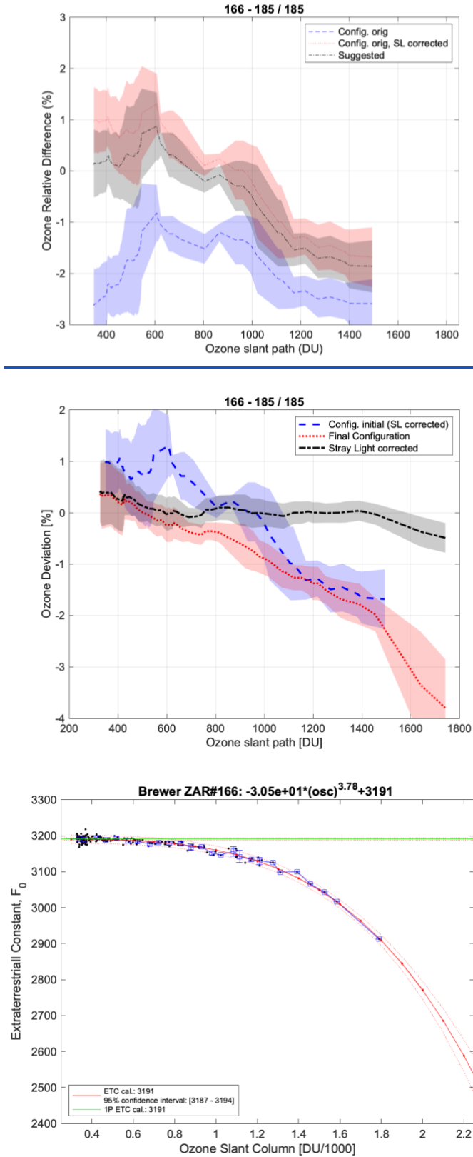
Figure 60. (Top) Ratio with respect to the reference used in the initial configuration with and without standard lamp correction. (Middle) Initial and final configuration with and without stray light correction. (Bottom) Stray light empirical model determination for B#166.
