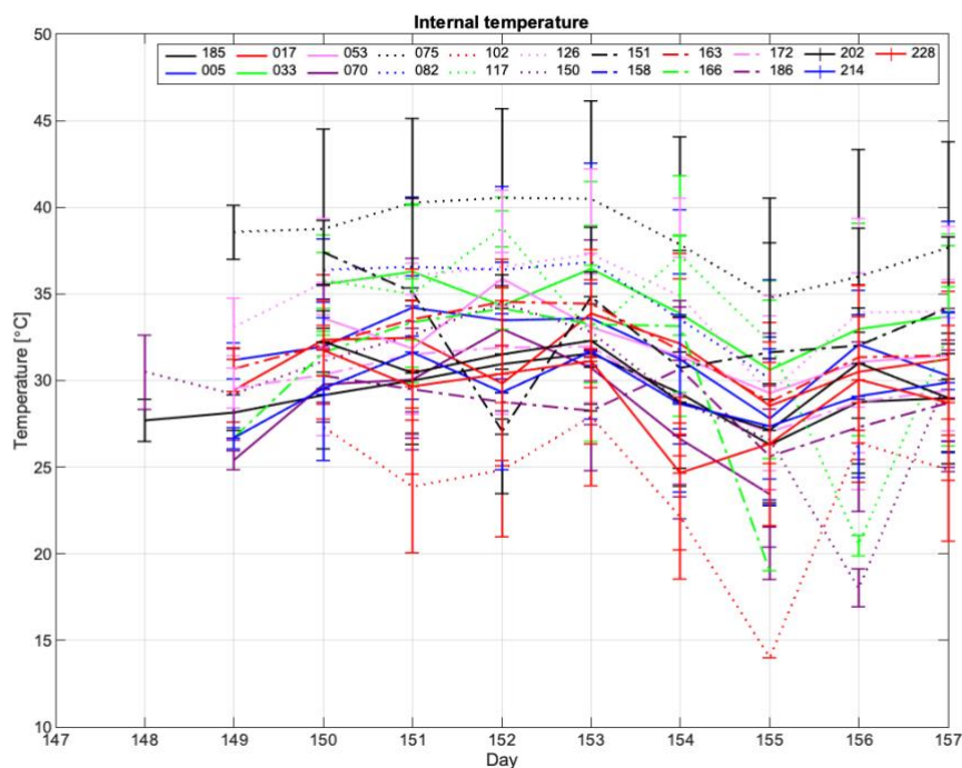
Figure 7. Statistics of the intercomparison conditions: internal temperature variability for all participating instruments
