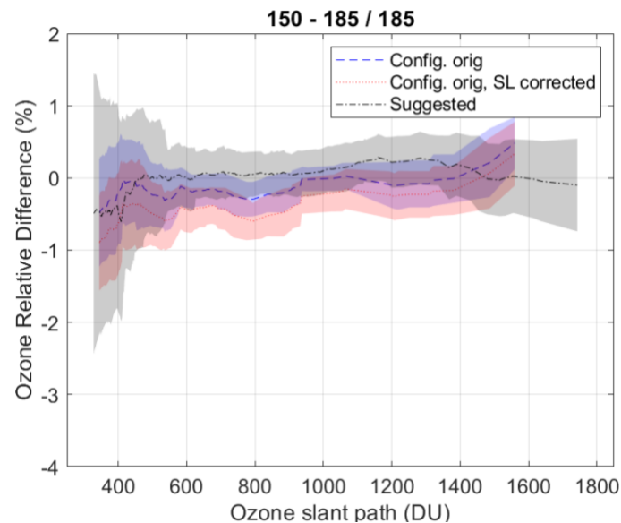
Figure 51. Ratio with respect to the reference using the initial configuration with and without the lamp correction, and the final configuration for B#150
