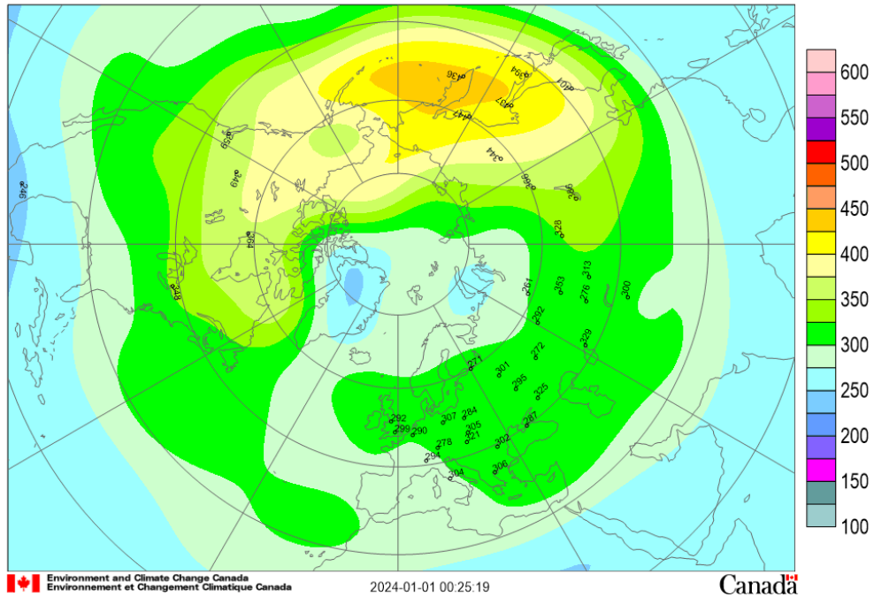
Mean total ozone (DU), 2023/12/01-2023/12/31
