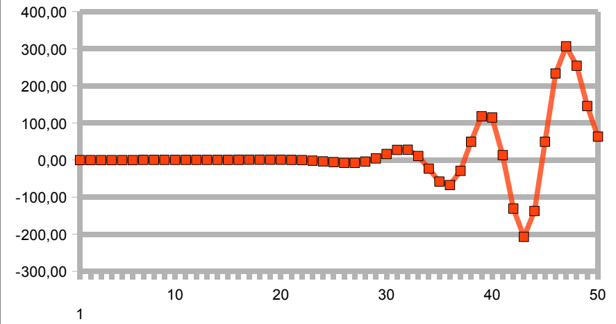
ERROR ABS L SIN( 6 PI x )
