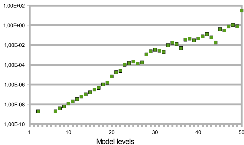
ERROR ABS L SIN( 6 PI x )
