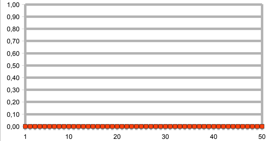
ERROR (G+S-GS-N) SIN( 6 PI x )
