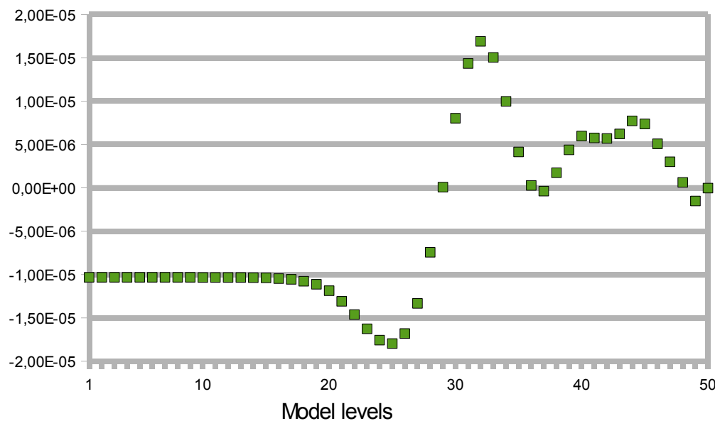
ERROR (G+S-GS-N) SIN( 6 PI x )
