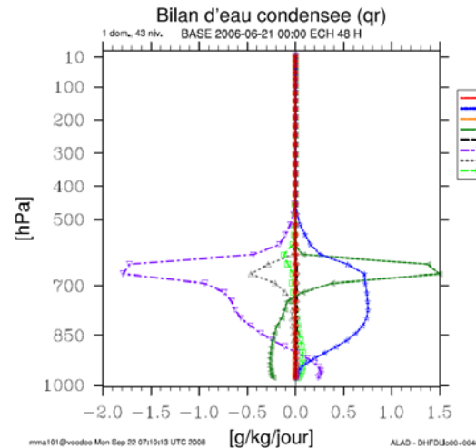
ARPEGE processes
