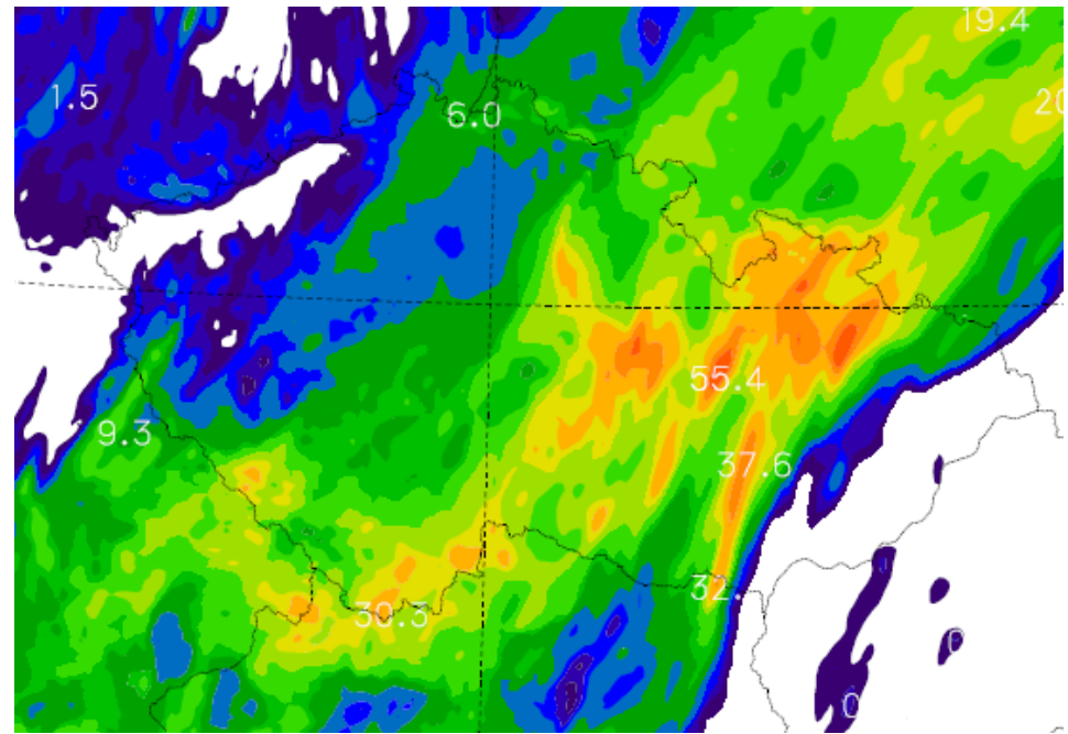
Grad (RT) with all species
