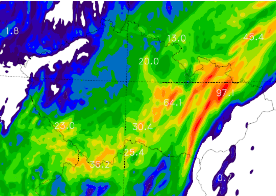
Grad (RT) with qv only; dx = 2.3km
